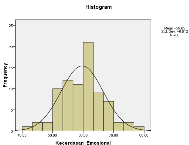
Figure 1. Histogram of emotional intelligence variables
