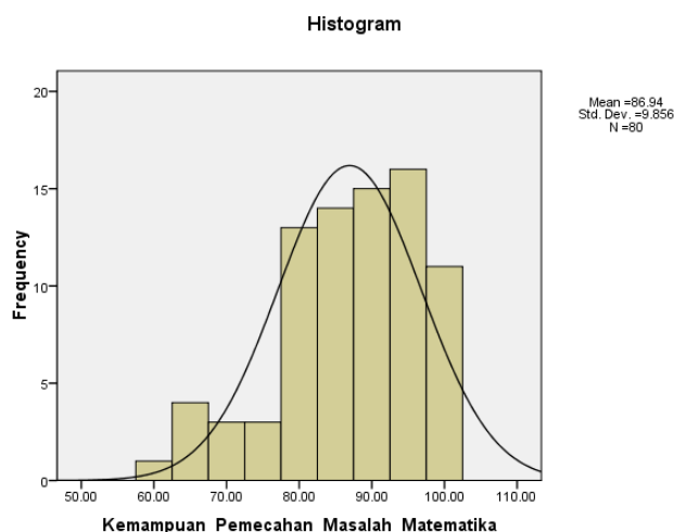
Figure 2. Histogram of Mathematics Problem Solving Ability Variable
