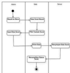
Gambar 6. Activity Diagram Admin Surat Masuk
