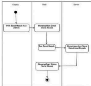
Gambar 8. Activity Diagram Manager Surat Masuk
