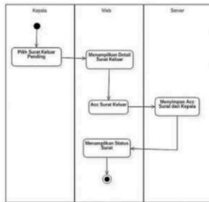
Gambar 7. Activity Diagram Manager Surat Keluar
