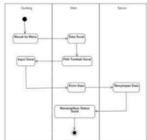
Gambar 9. Activity Diagram Gudang
