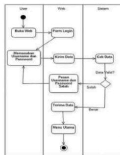
Gambar 3. Activity Diagram Login
